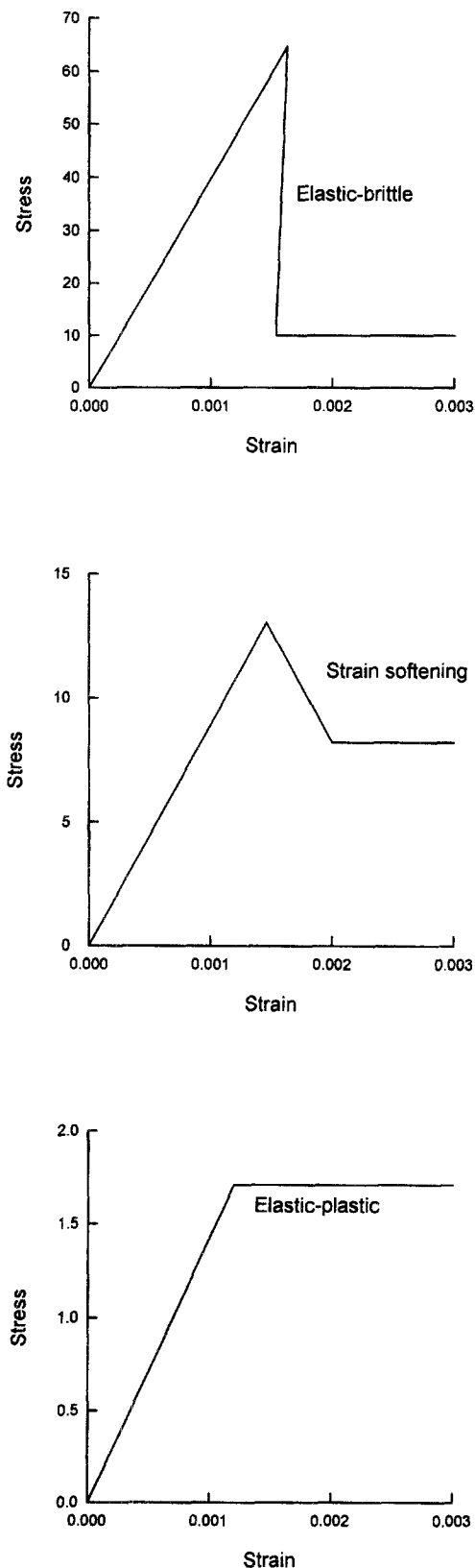
Fig. 9. Suggested post-failure characteristics for different quality rock masses. Note that the stress scales are different. (a) Very good quality hard rock mass, (b) Average quality rock mass, (c) Very poor quality soft rock mass.
