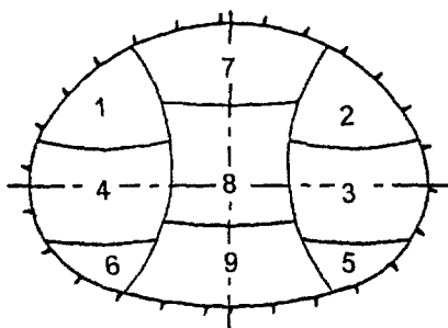
Fig. 17. Twin side drift and central pillar excavation method. Temporary support consists of double wire mesh reinforced 250–300 mm thick shotcrete shells with embedded lattice girders of HEB 160 steel sets at 0.75–1 m spacing.
