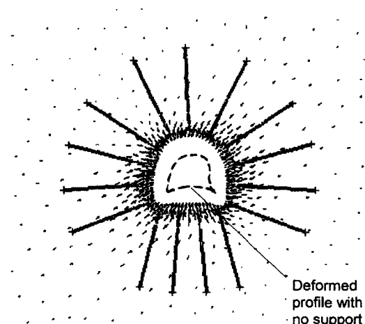
Fig. 22. Displacements in the rock mass surrounding the Yacambu-Quibor tunnel. The maximum calculated displacement is 258 mm with no support and 106 mm with support.
