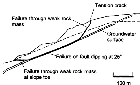
Fig. 24. Complex slope failure controlled by an outward dipping basal fault and circular failure through the poor quality rock mass overlying the toe of the slope.
