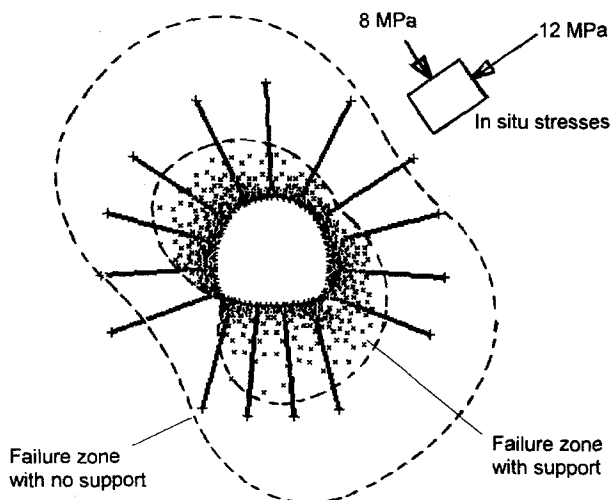
Fig. 21. Results of a numerical analysis of the failure of the rock mass surrounding the Yacambu-Quibor tunnel when excavated in graphitic phyllite at a depth of about 600 m below surface.
