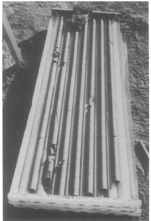
Fig. 12. Excellent quality core from a hard strong rock mass with very few discontinuities.
