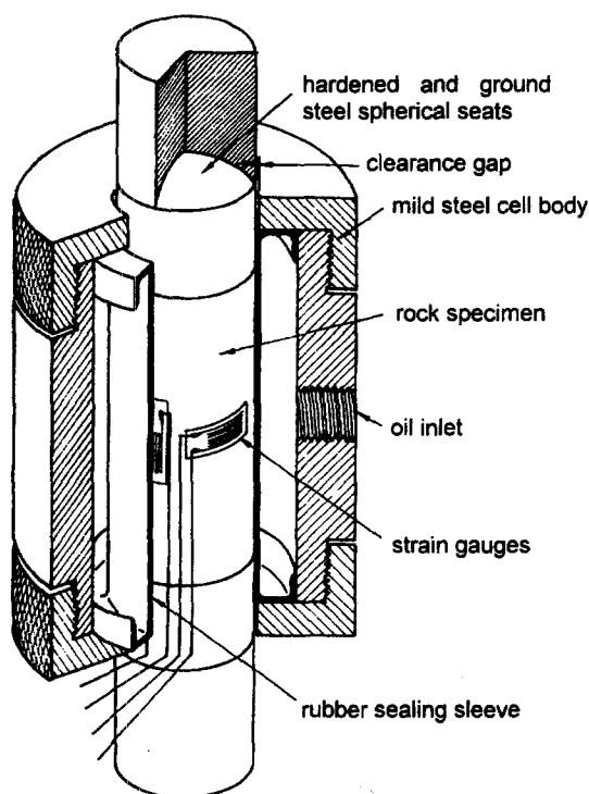
Fig. B1. Cut-away view of the triaxial cell designed by Hoek and Franklin [30].
