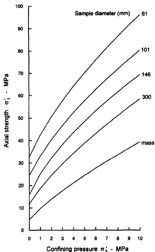
Fig. 3. Peak strength for Australian Moura coal. After Medhurst and Brown [10].
