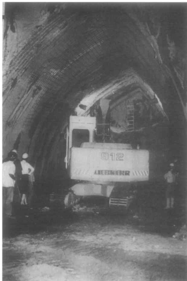
Fig. 19. Side drift in the Athens Metro Olypion station excavation, which was excavated by the method illustrated in Fig. 17. The station has cover depth of approximately 10 m over the crown.
