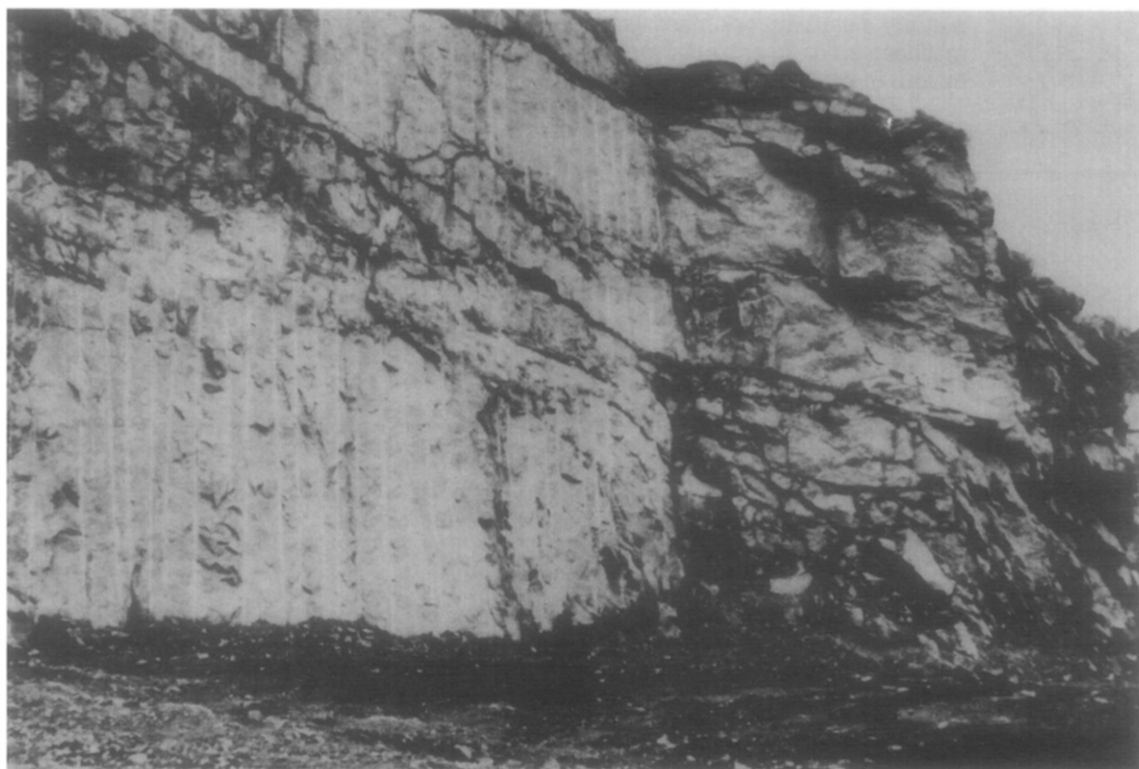
Fig. 5. Comparison between the results achieved by controlled blasting (on the left) and normal bulk blasting for a surface excavation in gneiss.
