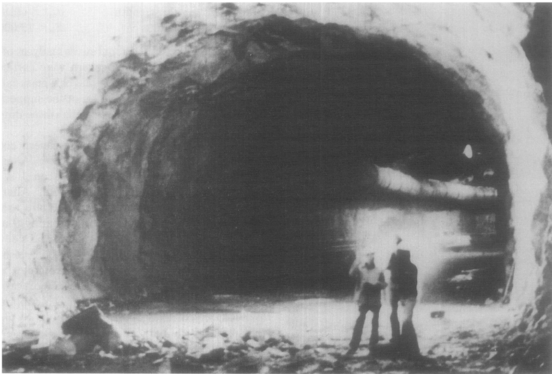
Fig. 13. Top heading for the 12 m span, 18 m high tailrace tunnel for the Rio Grande Pumped Storage Project.
